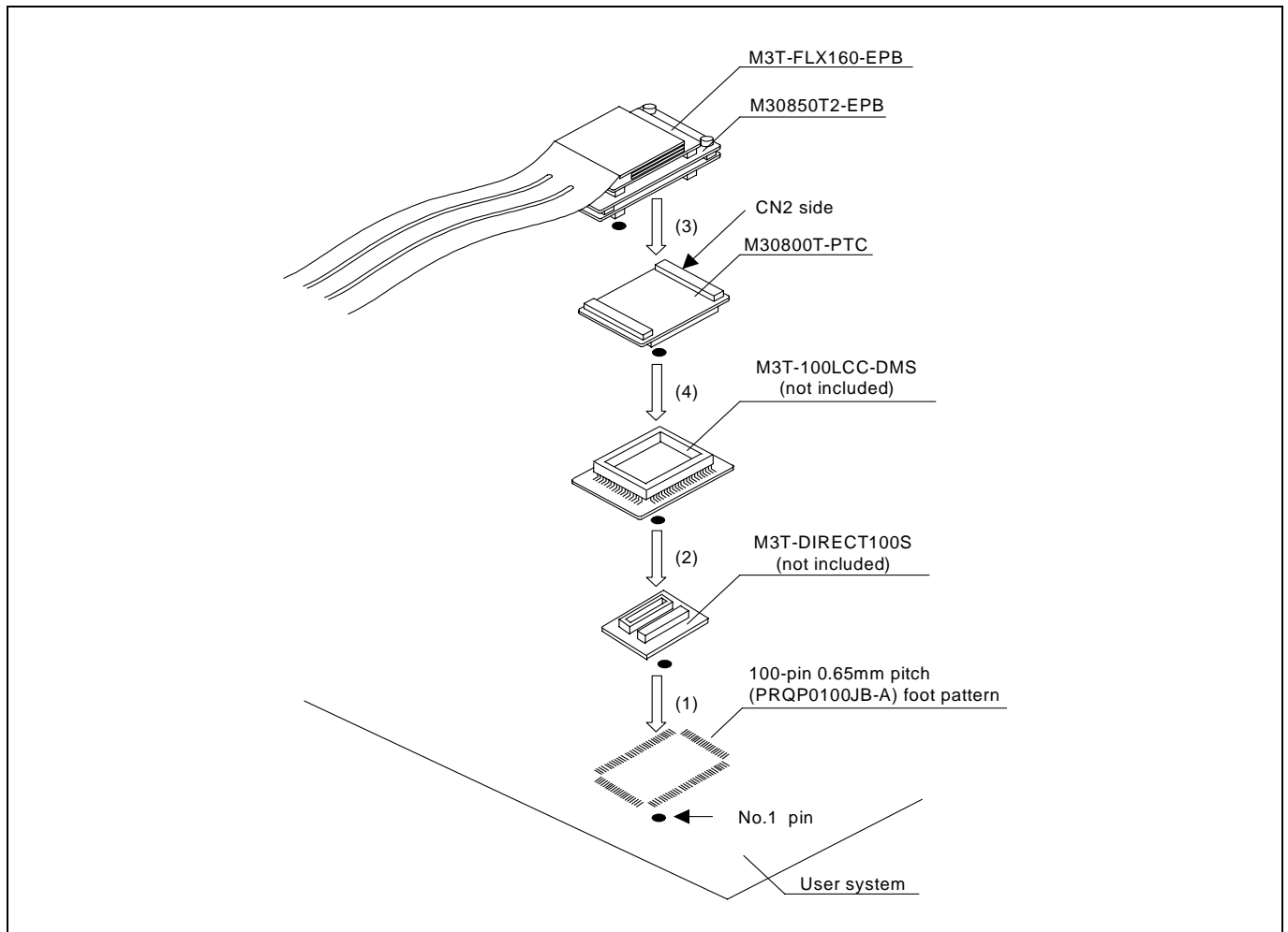
Figure 2.10 Connecting to a 100-pin 0.65mm pitch foot pattern (2/3)
